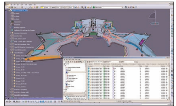
Pictured is a full aerodynamic design of the floor diffuser for Renault F1 Team's R29 race car during a CATIA V5 3D CAD modeling session. VISTAGY's FiberSIM® composites engineering software, which is fully integrated into the 3D CAD environment, enables Renault F1 Team to rapidly define the layup on a complex surface of a large amount of plies with multiple orientations and material types, thus ensuring part manufacturability in a timely fashion. The FiberSIM window in the lower right corner shows a list of ply layers sorted by sequence, step and name.
